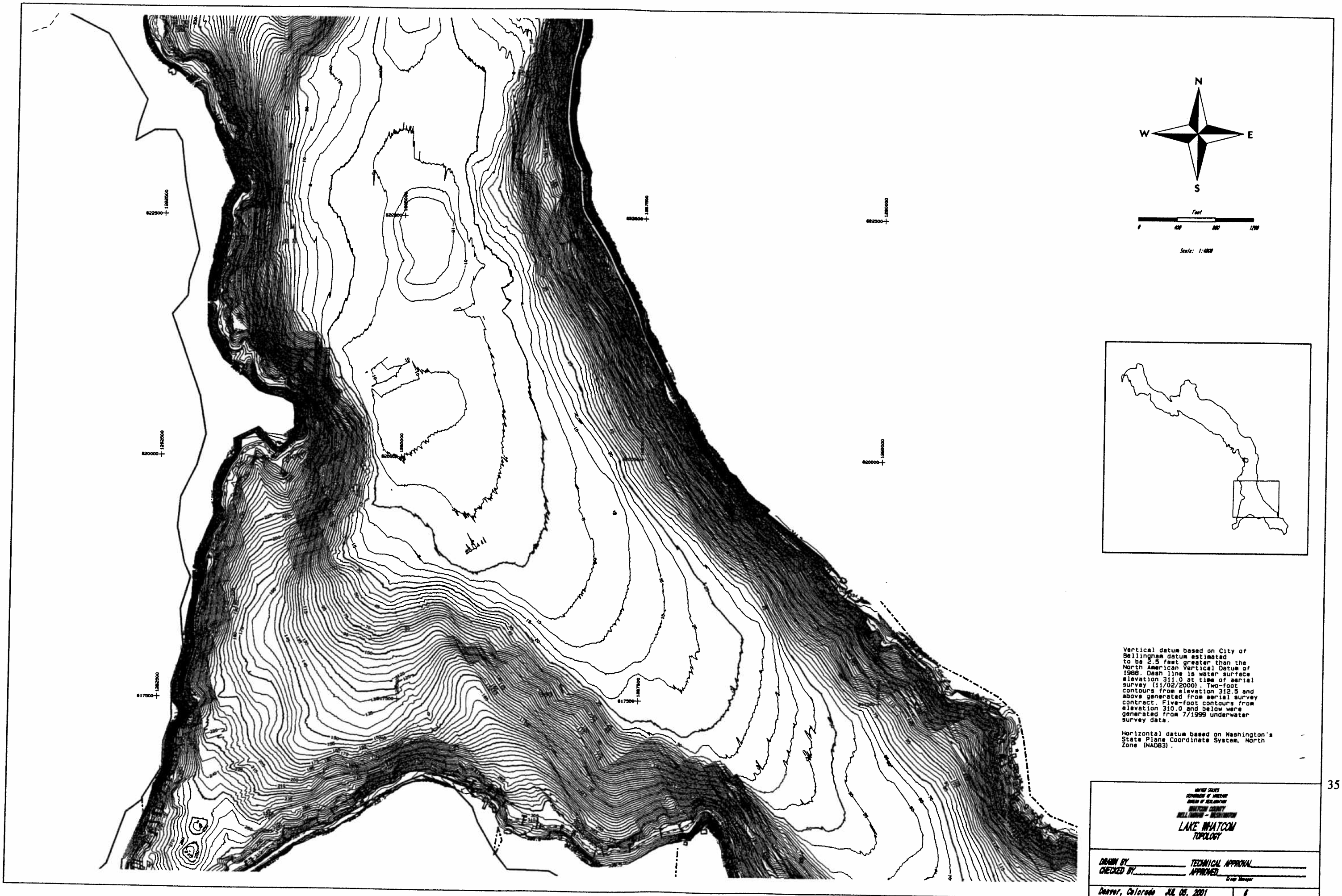
Figure 6. - Lake Whatcom topographic map, No. 6.
